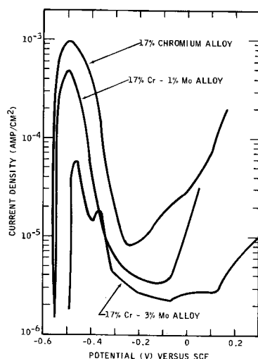
Fig. 2. Anodic potentiodynamic polarization curves for 17% chromium, 17% Cr-1% Mo, and 17% Cr-3% Mo alloys in 0.1N hydrochloric acid at 29.6°C (unmasked electrodes).
